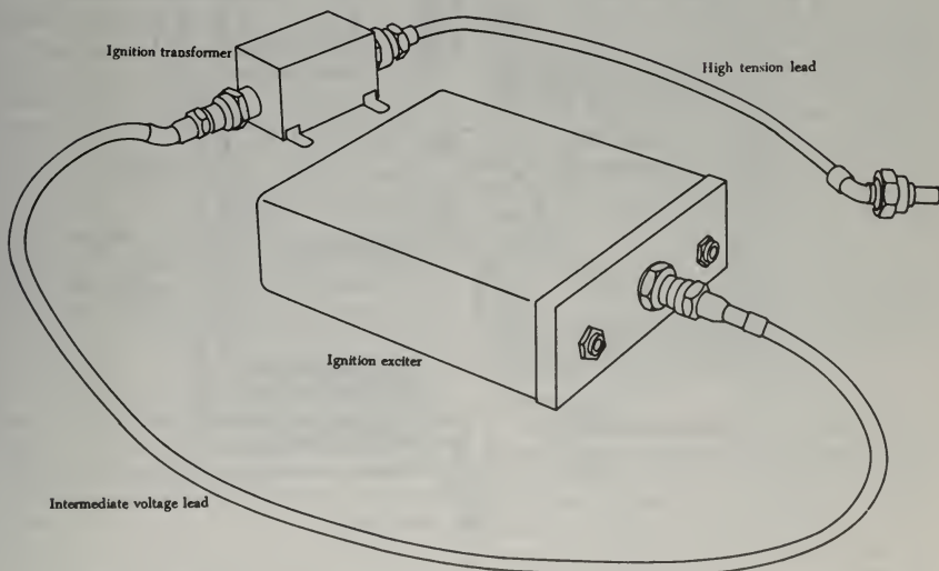
FIGURE 4-75. One side of a typical ignition system.
